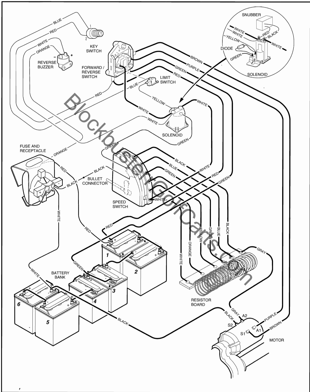
Figure 11-2 Wiring Diagram
