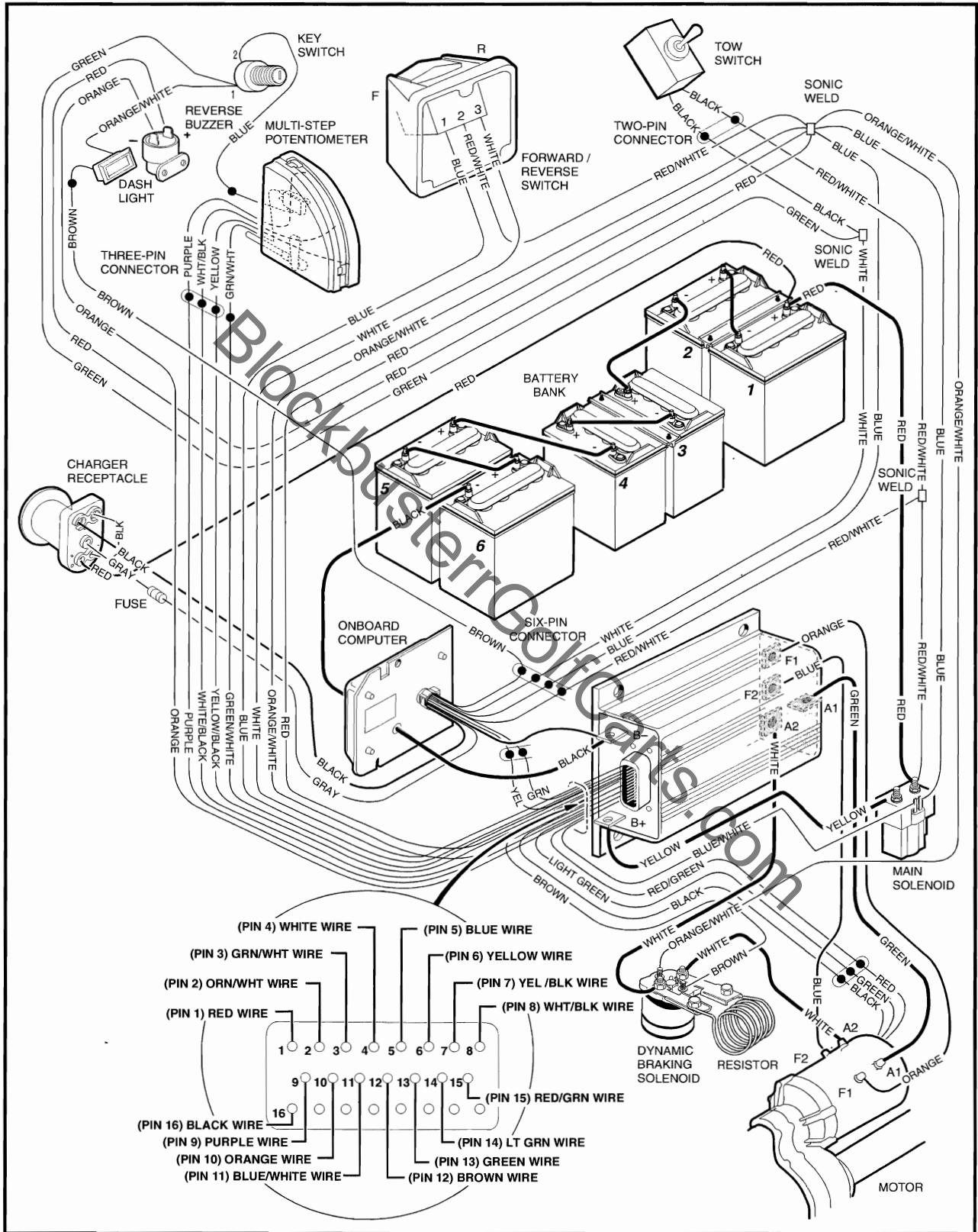
Figure 11-1 Wiring Diagram – Vehicle with Multi-Step Potentiometer
